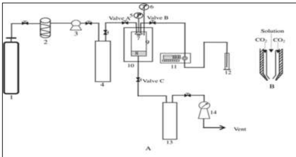
Figure No.1: Apparatus for preparing PLs by Supercritical Anti Solvent Method
